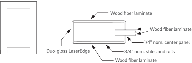
Shaker profile
